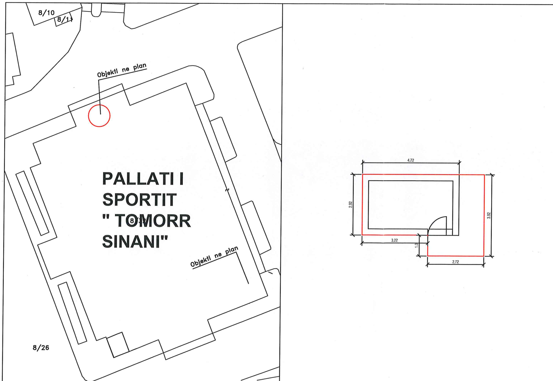
SHKALLA 1-100
