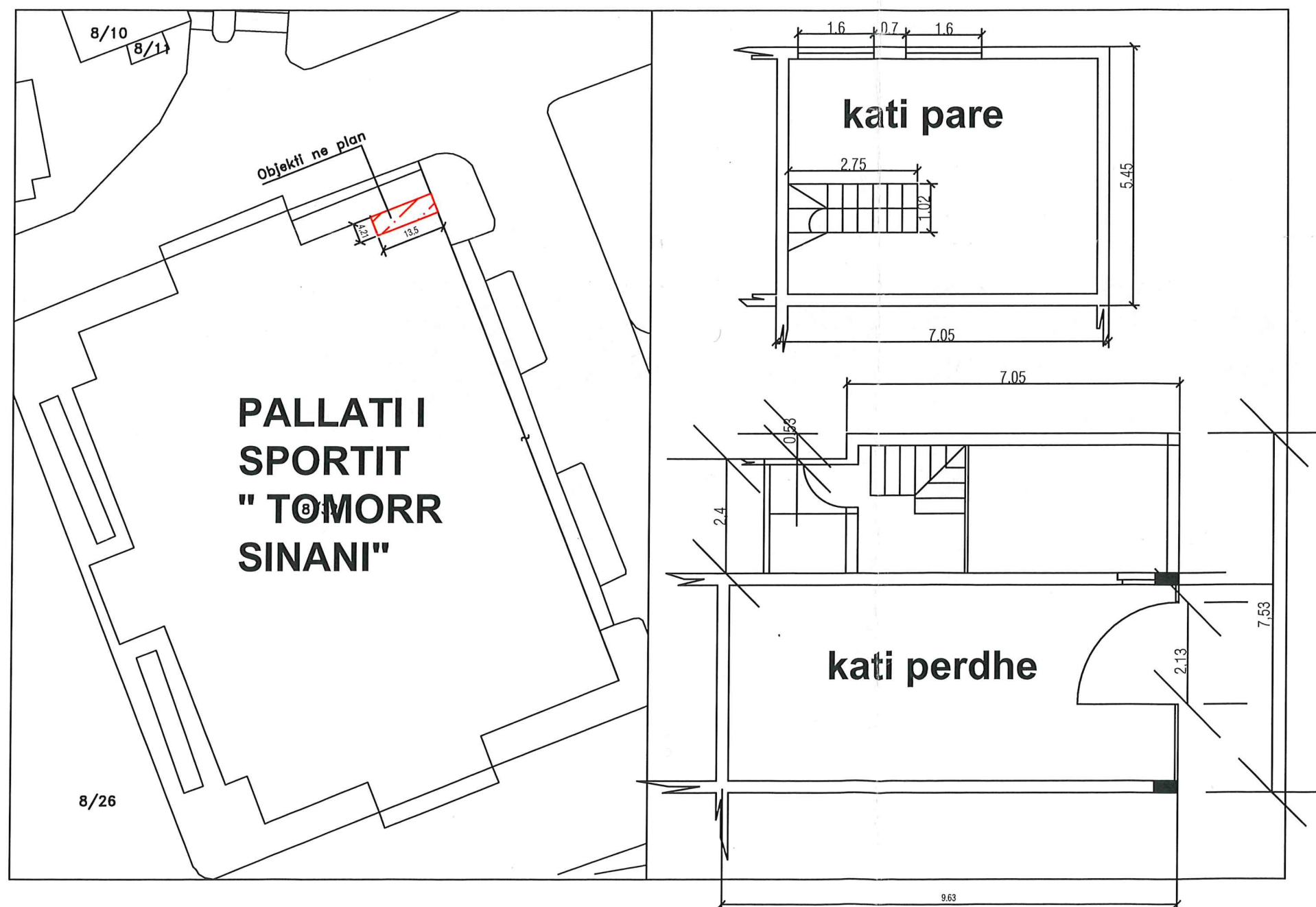
SHKALLA 1-100
